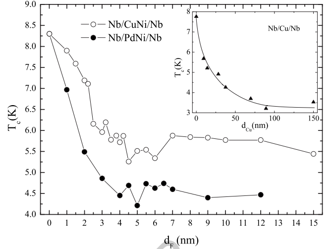
FIG. 1. Critical temperatures T_c versus the ferromagnetic layer thickness d_F for Nb/Cu 0.41 Ni 0.59 /Nb (open circles) and Nb/Pd 0.81 Ni 0.19 /Nb (closed circles) trilayers. Inset: T_c as a function of d_N in Nb/Cu/Nb system. The solid line is a guide to the eye.
