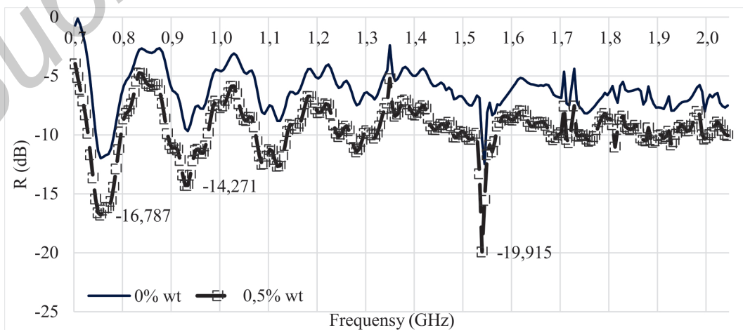
Fig. 6. Frequency dependences range from 0.7 GHz to 2 GHz of R_L for Fe_3O_4 nanoparticles and based sample of concrete at a thickness of 10 mm.
