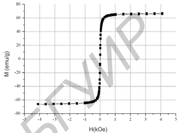
Fig. 5. Magnetic hysteresis of magnetite nanoparticles at room temperature.
