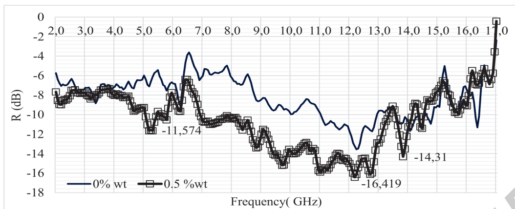
Fig. 7. Frequency dependences range from 2 GHz to 17 GHz of R_L for Fe_3O_4 nanoparticles and based sample of concrete at a thickness of 10 mm.
