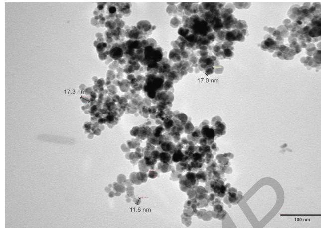
Fig. 3. TEM image of magnetite nanoparticles.
