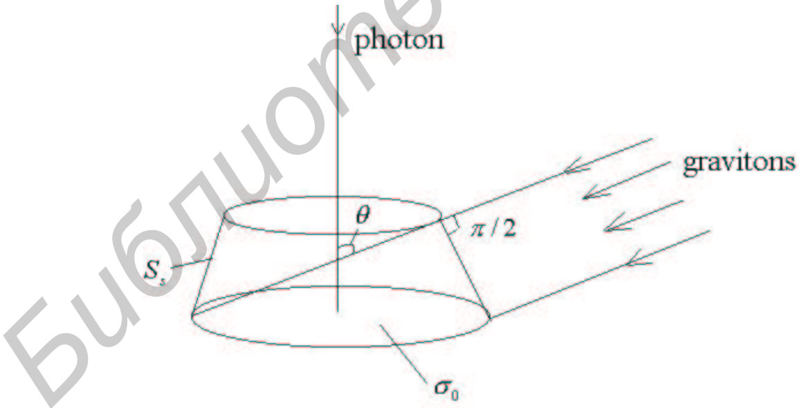
Figure 6.1: By non-forehead collisions of gravitons with a photon, it is necessary to calculate a cone's side surface square, S_s .
