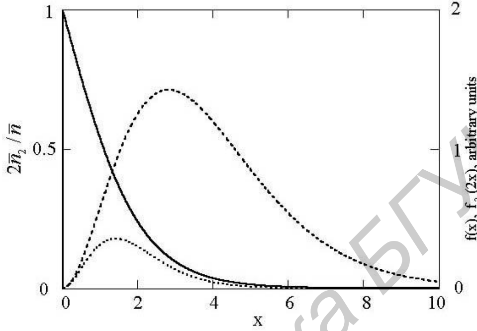
Figure 4.1: The portion of pairing gravitons, 2\bar{n}_2/\bar{n} , (solid line), a spectrum of single gravitons, f(x) , (dashed line), and a spectrum of graviton pairs, f_2(2x) , (dotted line) versus the dimensionless parameter x .
