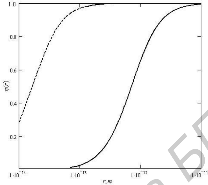
Figure 11.6: A non-universal transition to the limit value of unity of the function \eta(r) by E_2 = m_p c^2 (solid) and by E_2 = m_e c^2 (dot).
