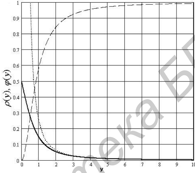
Figure 11.2: Graphs of the functions \rho(y) (solid), \rho(y)_d (dot), \varphi(y) (dash) .
