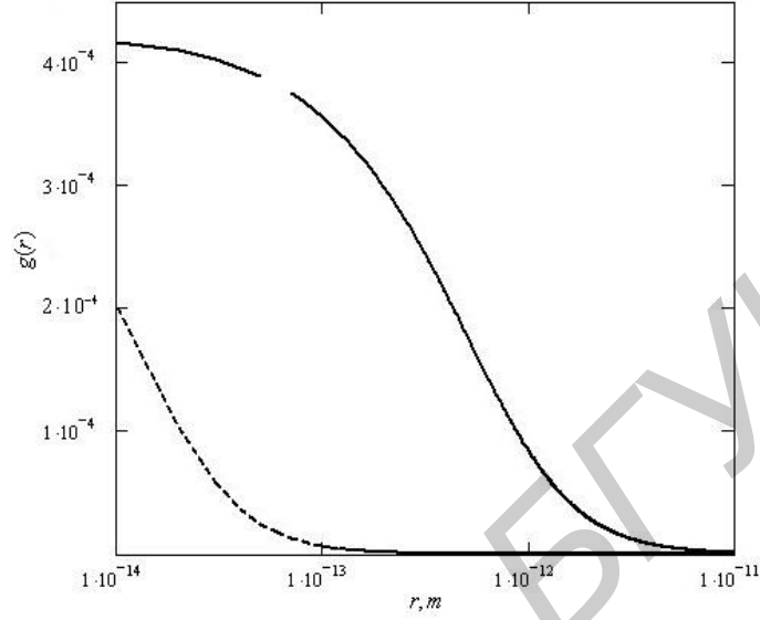
Figure 11.5: Different transition to the limit value of the function g(r) by E_2 = m_p c^2 (solid) and by E_2 = m_e c^2 (dot).
