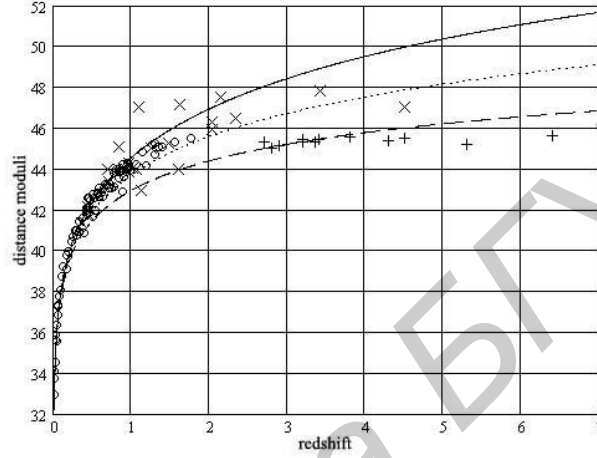
Figure 12.1: Hubble diagrams \mu_0(z) with b = 2.137 (solid), b = 1 (dot) and b = 0 (dash); supernova observational data (circles, 82 points) are taken from Table 5 of [10], gamma-ray burst observations are taken from [11] (x, 24 points) and from [12] (+, 12 points for z > 2.6 ).
