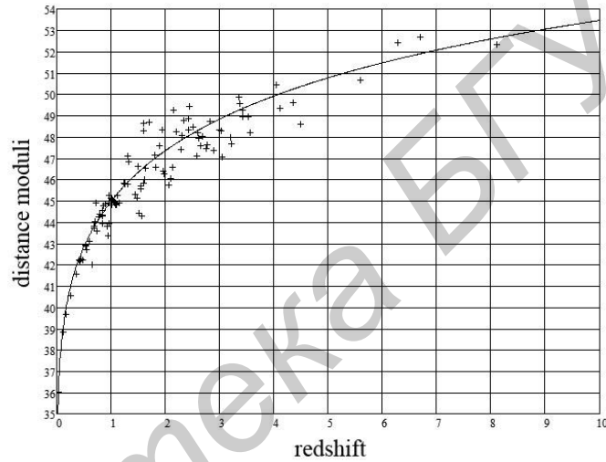
Figure 14.2: The theoretical Hubble diagram \mu_0(z) of this model with b = 2.137 (solid); GRBs calibrated observational data (pluses, 109 points) from Tables 1 and 2 of [9] corrected for no time dilation.
