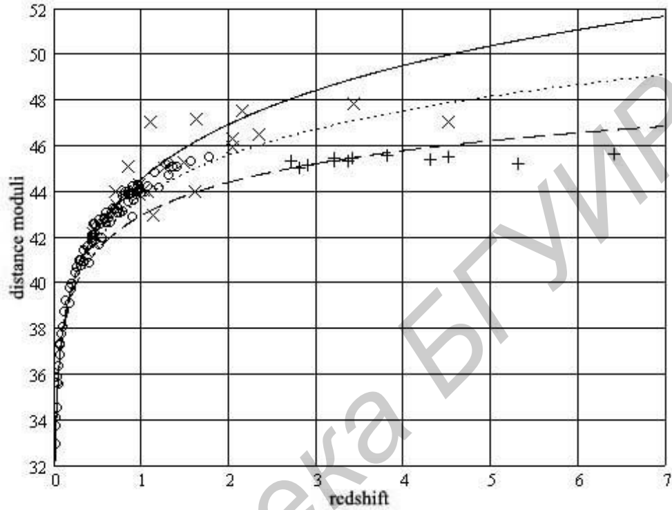
Figure 9.1: Hubble diagrams \mu_0(z) with b = 2.137 (solid), b = 1 (dot) and b = 0 (dash); supernova observational data (circles, 82 points) are taken from Table 5 of [5], gamma-ray burst observations are taken from [6] (x, 24 points) and from [7] (+, 12 points for z > 2.6 ).
