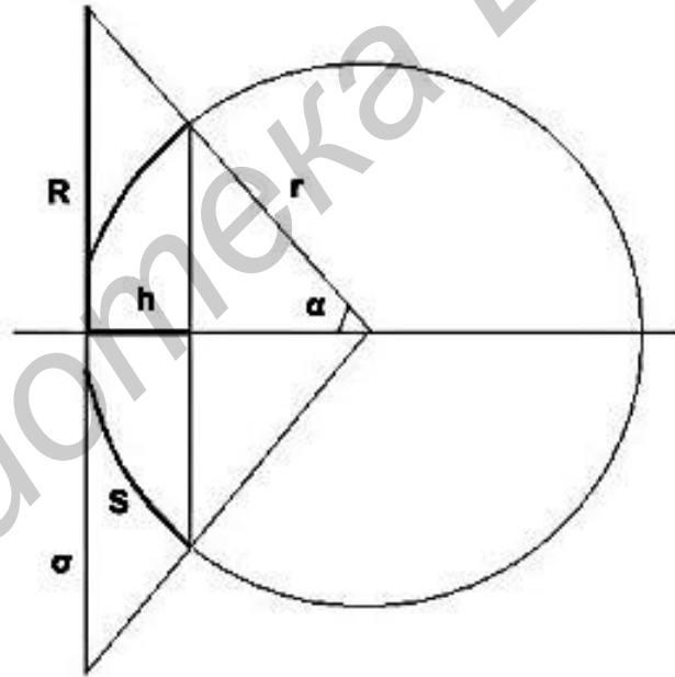
Figure 11.1: To the computation of the screened portion of gravitons at small distances: \sigma is the cross-section, S is a square of the spherical segment of a height h .
