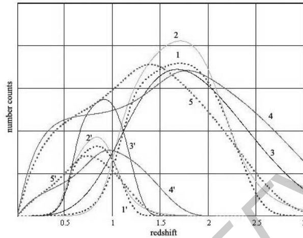
Figure 12.3: QSO number counts f_5(m, z) (arbitrary units) as a function of the redshift for different luminosity functions: Gaussian (1', 1 dot), the double power law (2', 2), Schechter's (3', 3), combined (4', 4 solid and 5', 5 dot) with parameters given in the text of [9]. The left-shifted curve of each couple (1' - 5') corresponds to the range 16 < m < 18.25 , another one (1 - 5) corresponds to 18.25 < m < 20.85 .
