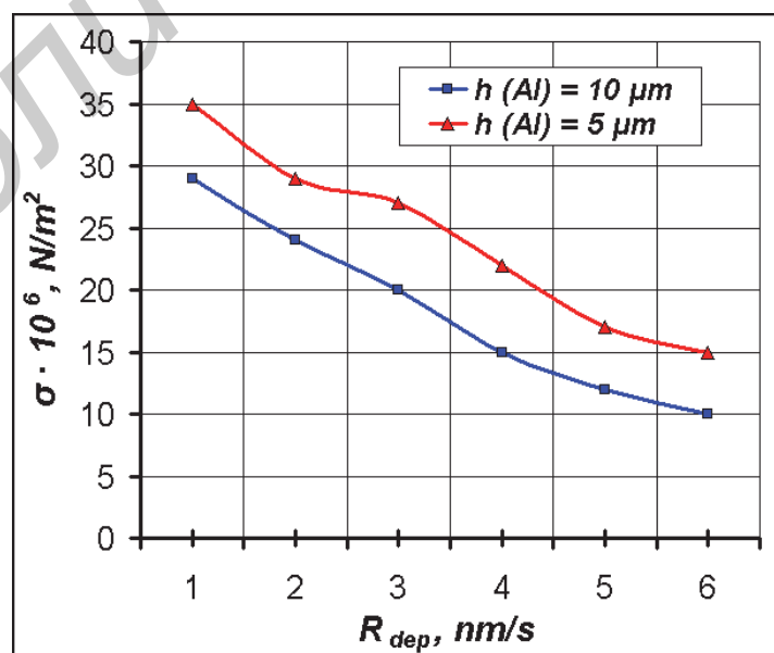
Fig. 2. Dependence of the internal stresses on the deposition rate of the aluminum films.
