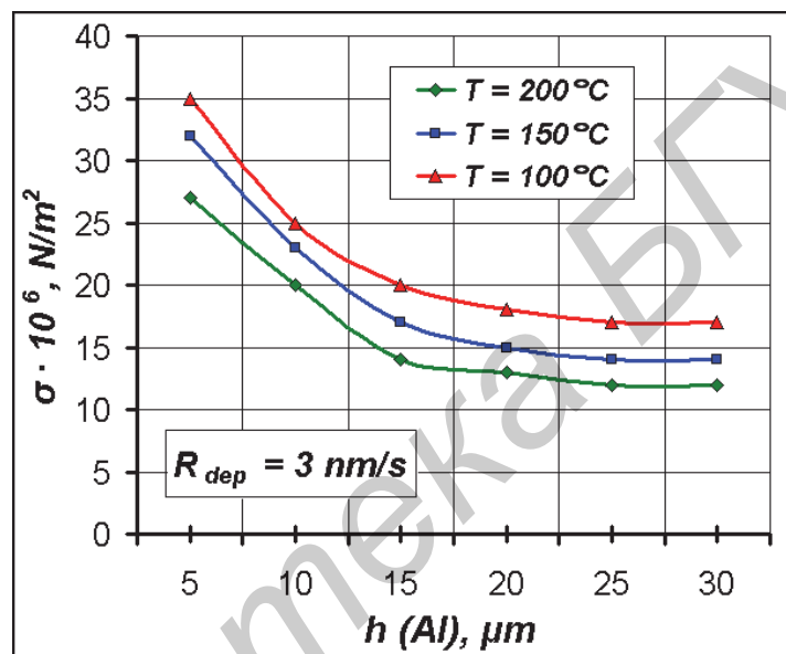
Fig. 1. Dependence of the internal stresses on the thickness of the aluminum films at various substrate temperatures.
