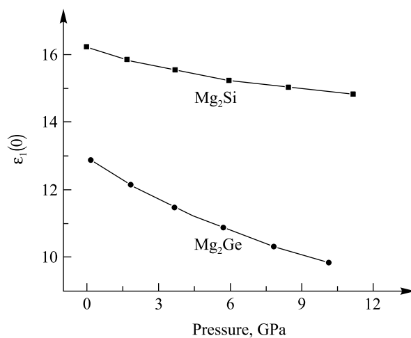
Fig. 5. Static dielectric function \epsilon_0 of Mg 2 Si and Mg 2 Ge as a function of the hydrostatic pressure
