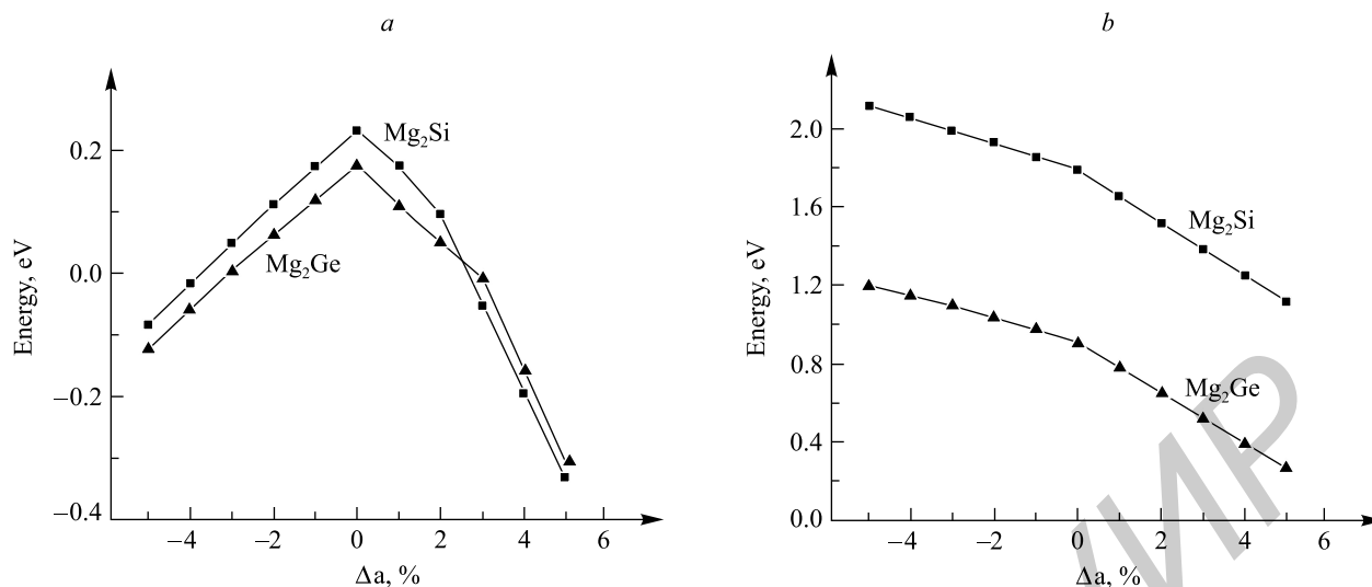
Fig. 7. The behaviour of the main interband transitions in Mg_2Si and Mg_2Ge under the uniaxial deformation: a – for indirect gap; b – for direct gap
