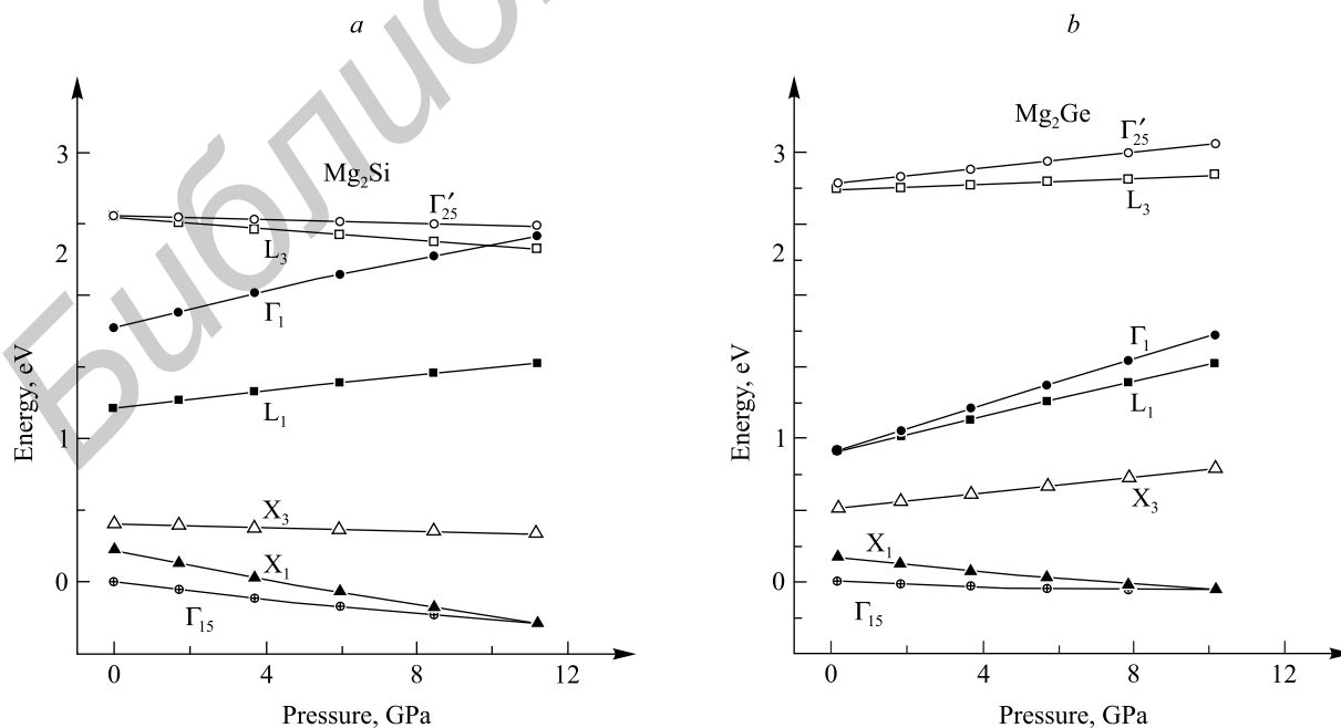
Fig. 2. Energies of the top valence and the two lowest conduction states of Mg 2 Si ( a ) and Mg 2 Ge ( b ) at some k -points as a function of hydrostatic pressure
