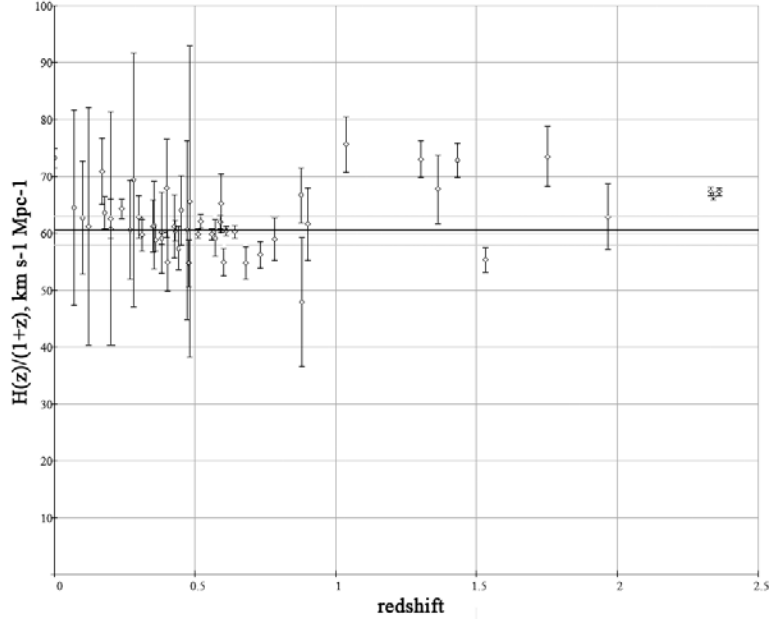
Figure 2: The ratio H(z_i)/(1+z_i) \pm \sigma_{0i} and the weighted value of the Hubble constant \langle H_0 \rangle \pm \sigma_0 (horizontal lines); 51 H(z) observational data points are taken from Table 1 of [6].
