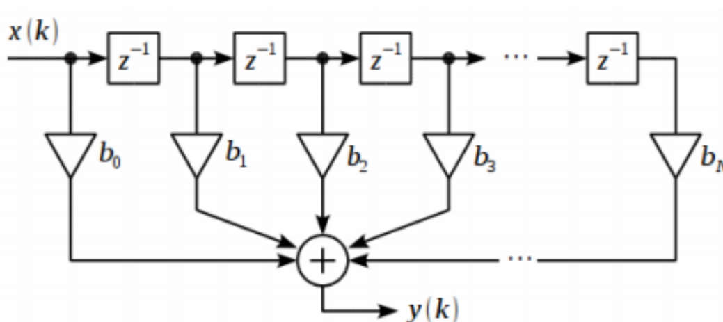
Fig. 1 – Block diagram of a non-recursive FIR filter
