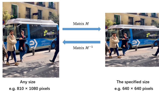
Figure 2 Image transformation
