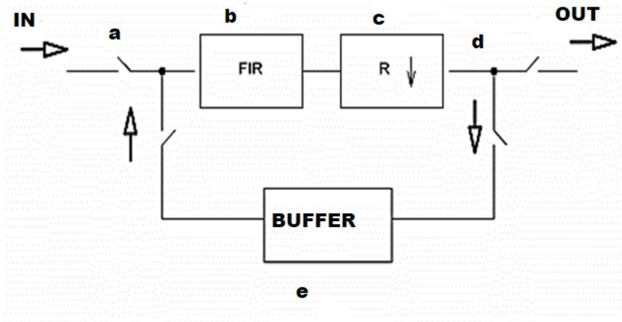
Fig. 2 – Block diagram of the buffer FIR filter:
