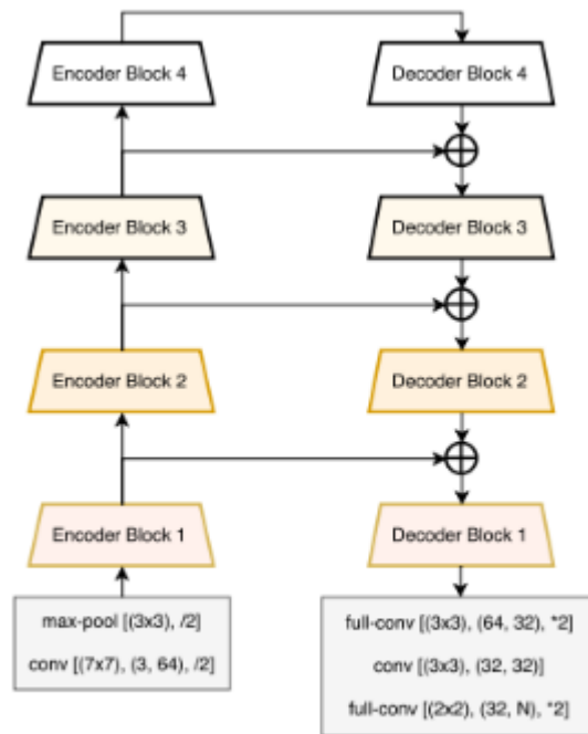
Fig. 1: LinkNet Architecture
