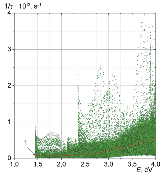
Fig. 2. Scattering rates for the acoustic mode TA on energy
