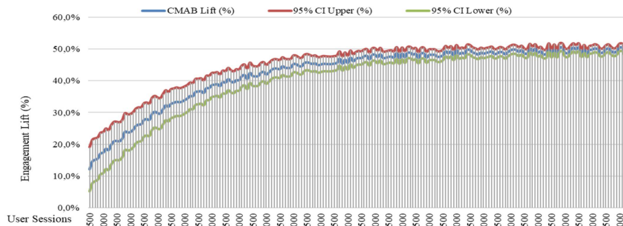
Figure 4. Engagement Lift over Baseline (%)
