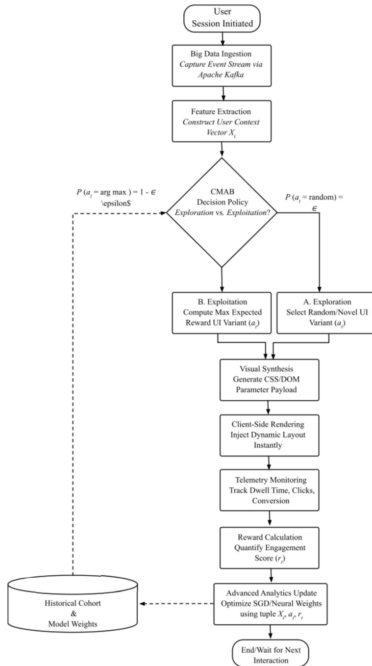
Figure 2. Algorithmic Trace of the Contextual Multi Armed Bandit Policy for Real Time UI-Personalization
