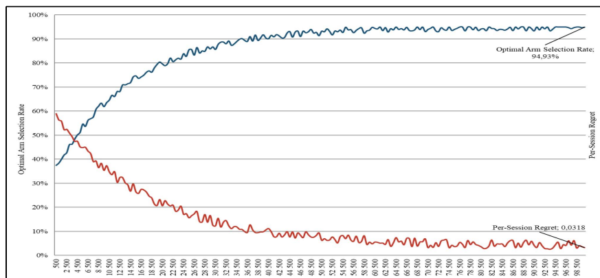
Figure 5. Optimal Arm Selection Rate & Per-Session Regret
