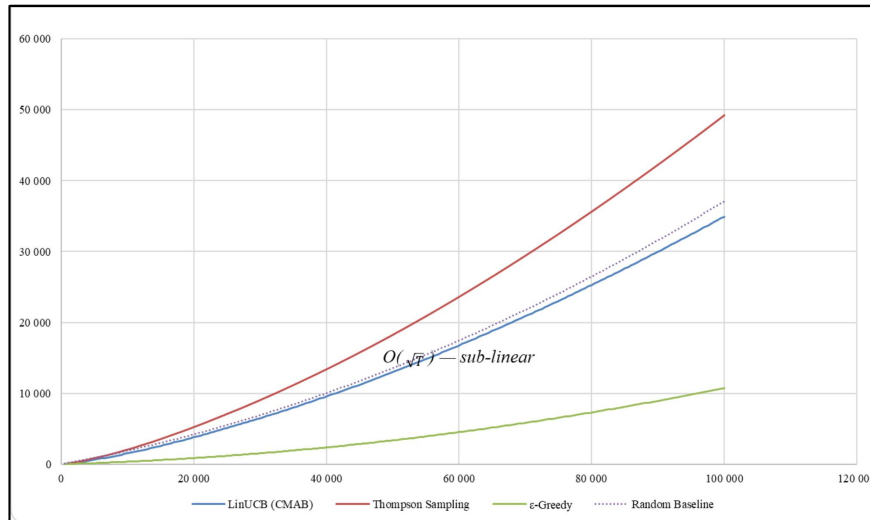
Figure 3. Cumulative Regret - Algorithm Comparison
